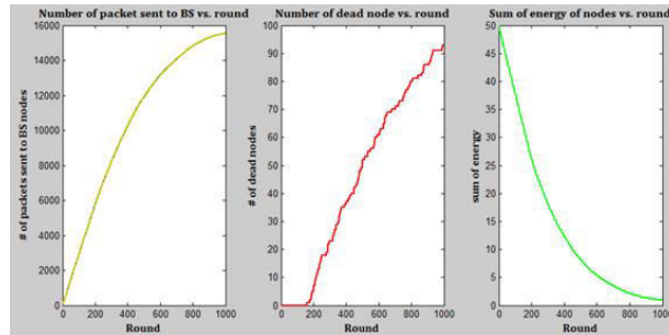
Figure 6: PDR, DN and E versus 1000 Round
