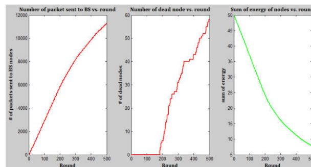
Figure 4: PDR, DN and E versus 500 Round
