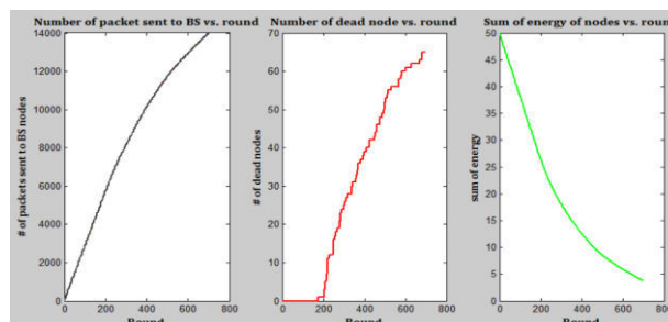
Figure 5: PDR, DN and E versus 700 Round
