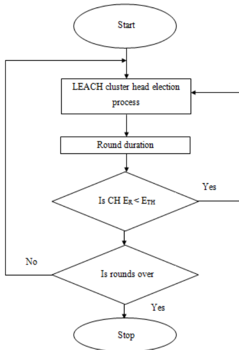
Figure 2: Dynamic Cluster Head Election Algorithm
