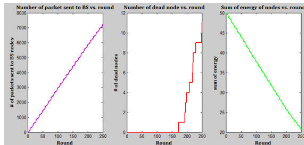
Figure 3: PDR, DN and E versus 250 Round
