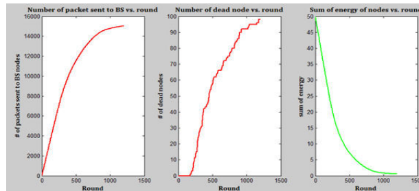
Figure 7: PDR, DN and E versus 1200 Round
