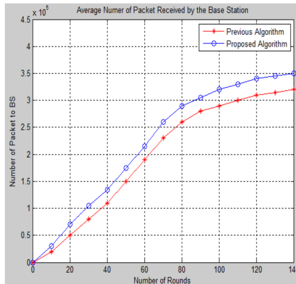
Figure 12: Average number of packet received by the base station
